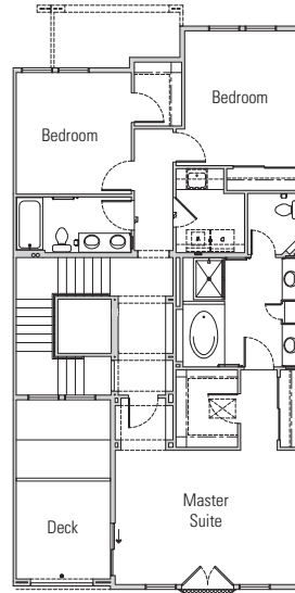
THIRD FLOOR
